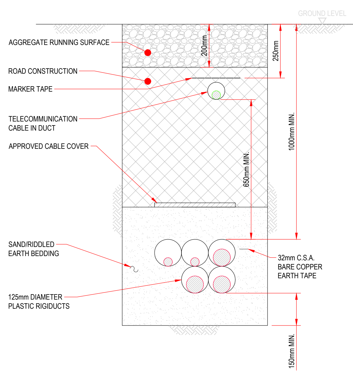
3-33kV CABLES ROAD CROSSING SECTION
